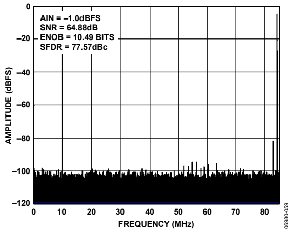
Figure 4. Single-Tone 32k FFT with f_{IN} = 84.3 MHz, f_{SAMPLE} = 170 MSPS
